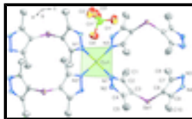
Fig. 1. A portion of the crystal structure of the title compound showing the labeling scheme and 50% probability displacement ellipsoids [symmetry codes: (i) -x, 1-y, -z , (ii) -x, y, -0.5-z , (iii) x, 1-y, -1/2+z ]. H atoms are omitted for clarity.
